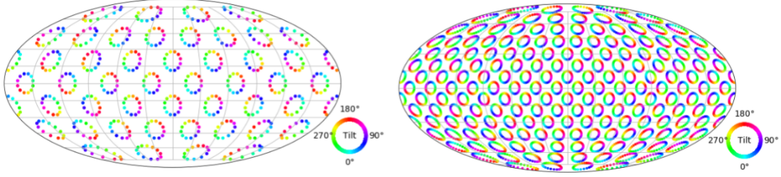
Figure 4.2: Equi-Volumetric Sampling of \text{SO}(3) . The normalization term is approximated by computing the unnormalized probabilities on an equi-volumetric grid. The method proposed by [21] produces equal-area grids hierarchically on the 2-sphere using the HEALPix method [20] and finally samples rotations using the Hopf fibration [22]. Left: a grid with 576 rotations, right: 4608 rotations [5].
